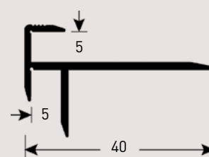
Double edge nosing, decoration series (aluminium)* Ref. 1605
